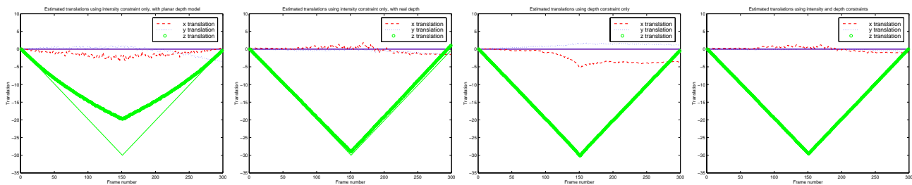
Figure 3. Comparison of ground truth (solid) with computed perspective translation parameters (see legend) for synthetic Z-translation sequence. Left: BCCE only with planar depth model; Middle-left: BCCE only with real depth; Middle-right: DCCE only; Right: Both constraints used.
